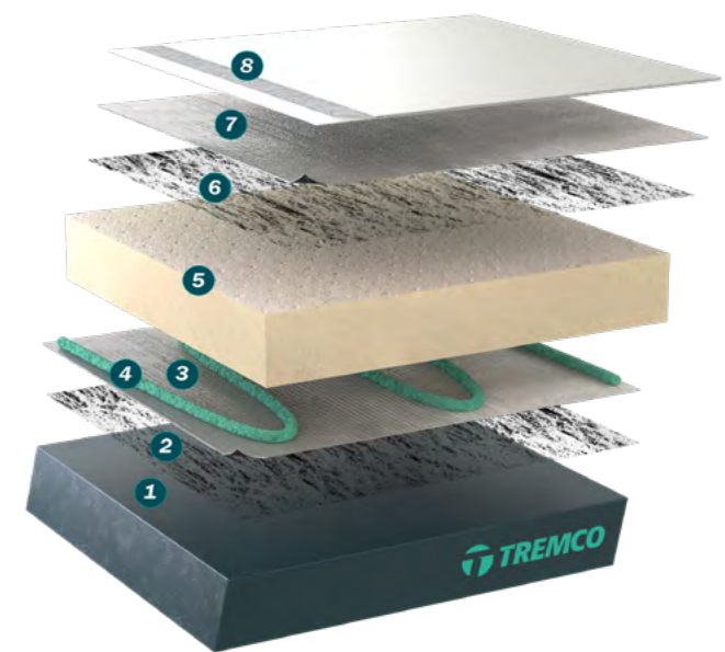
Warm roof application
