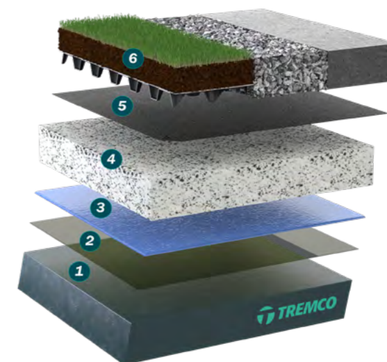
Warm roof application
