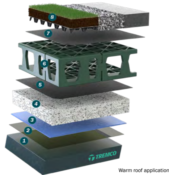
Warm roof application
