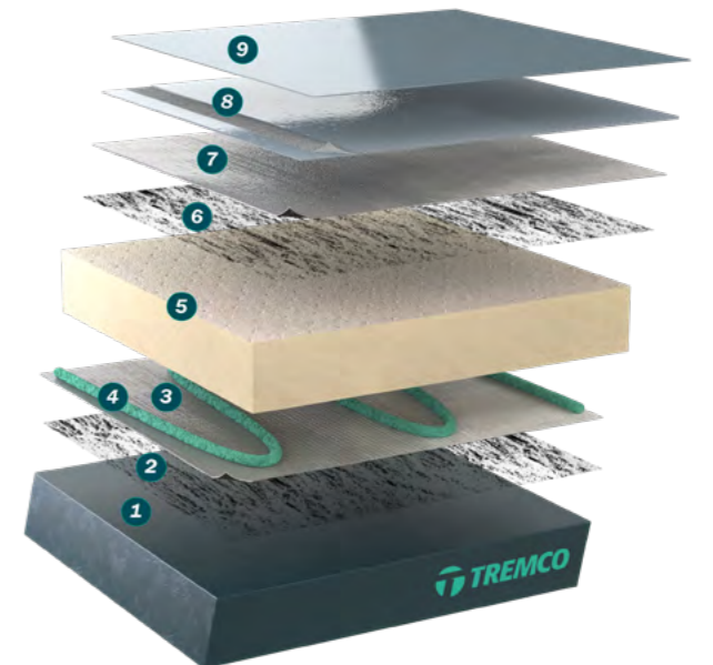
Warm roof application
