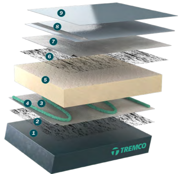
Warm roof application
